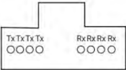
40G Base-SR4 8-Fiber and 100G Base-SR4 8-Fiber MTP (1) 8 strand MTP trunk is used for one link.
