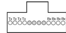
40G BASE-SR4 8-Fiber and 100G BASE-SR4 8-Fiber MTP (1) 8 strand MTP trunk is used for one link
