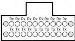
100G Base-SR10, 1 x 24-Fiber MTPs with the 100G option (1) 24 strand MTP trunks are used for one link.
