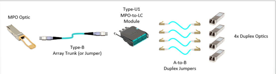
Figure 2: Breakout Application via Type-U1 MPO-to-LC Module
