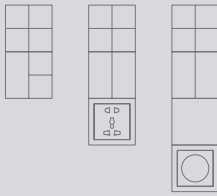
Vertical multi-gang installation
